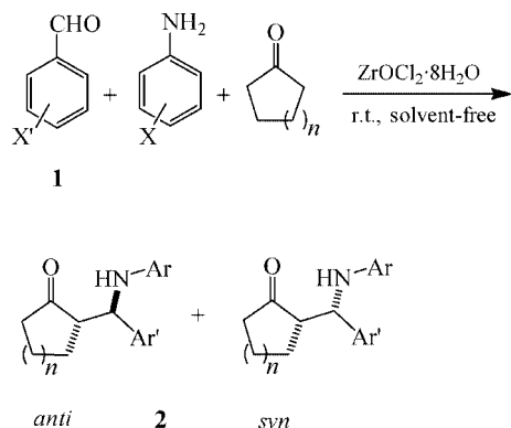
Scheme 1. Direct Mannich-type reaction between aldehydes of type 1 , anilines, and cyclic ketones.
