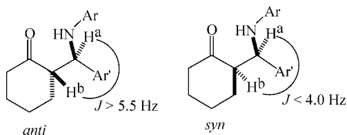
Scheme 5. Identification of anti and syn isomer by ^1\text{H} NMR spectroscopy.
