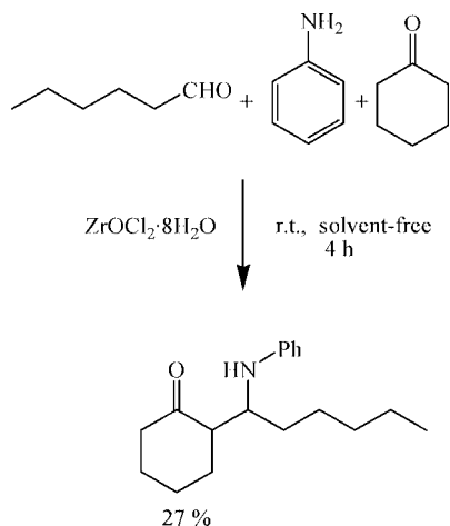
Scheme 4. Reaction conditions: to aniline (1 mmol), hexanal (1 mmol), cyclohexanone (3 equiv.), and \text{ZrOCl}_2 \cdot 8\text{H}_2\text{O} (0.05 g) were added successively at room temp. and stirred for 4 h.
