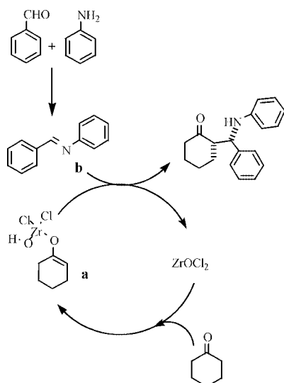
Scheme 2. Proposed reaction mechanism for Mannich reactions of benzaldehyde, anilines, and cyclohexanone.
