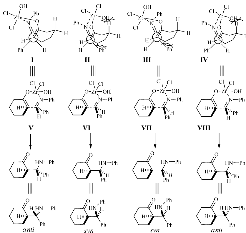
Scheme 3. Four possible transition states.
