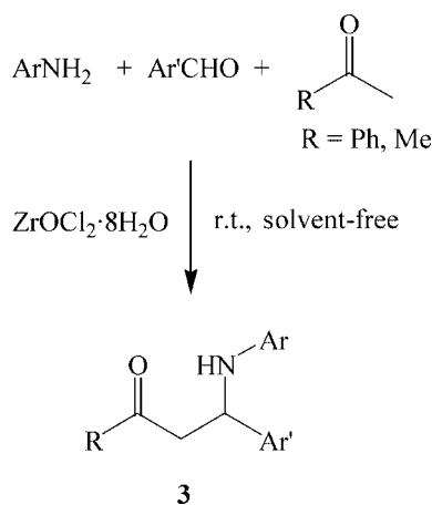
Scheme 6. Mannich reaction of aromatic aldehydes, anilines, and acyclic ketones.
