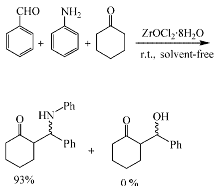
Scheme 7. Chemoselectivity of cyclohexanone toward aldimine in preference to aldehydes.
